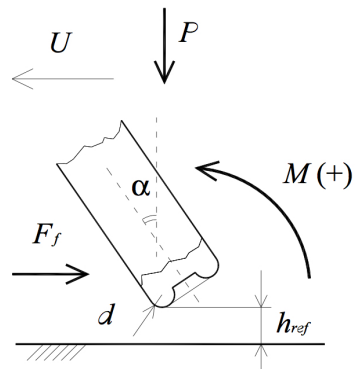
Schematic view of the tip-glass contact
